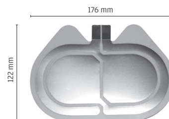
812-80H Disposable neutral electrode EMED SAFE, hydrogel, split, for adults and children 176x122mm, 110 cm 2 , 10x5pcs.
